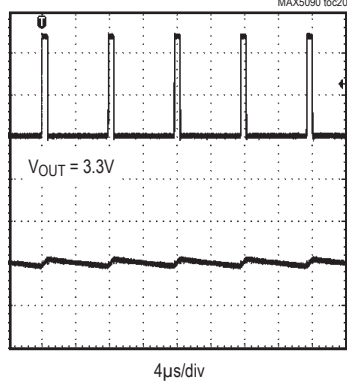
A: SWITCH VOLTAGE (LX PIN), 20mV/div ( V_{IN} = 48V ) B: INDUCTOR CURRENT, 2A/div ( I_O = 2A )
