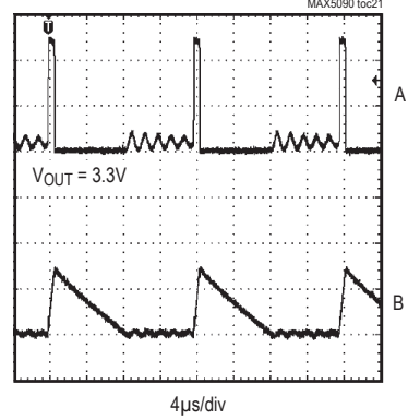
A: SWITCH VOLTAGE, 20V/div ( V_{IN} = 48V ) B: INDUCTOR CURRENT, 200mA/div ( I_O = 75mA )
