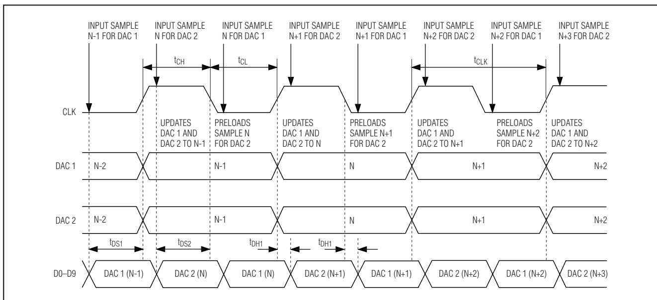
Figure 4. Timing Diagram
