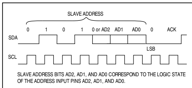
Figure 5. Address Byte
