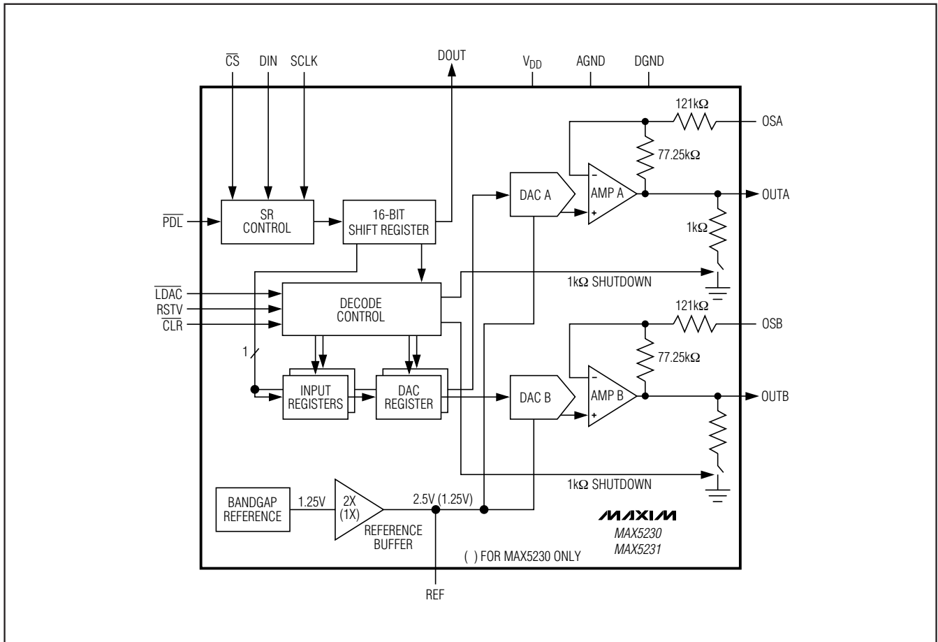
Functional Diagram
