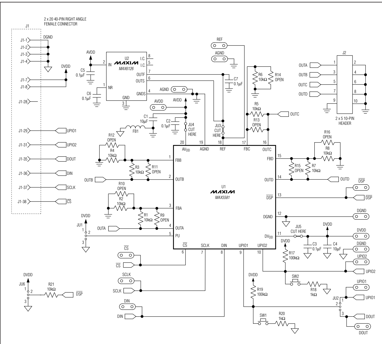
Figure 11. MAX5581 EV Kit Schematic
