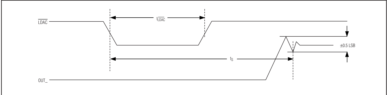
Figure 2. LDAC Timing
