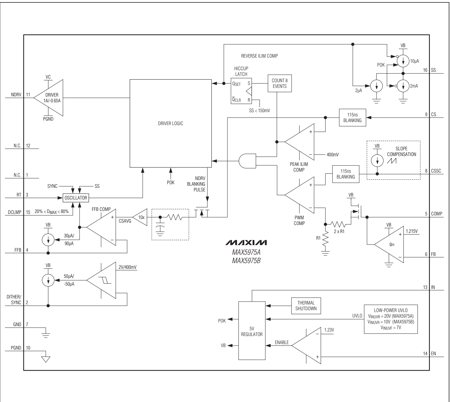
Block Diagram
