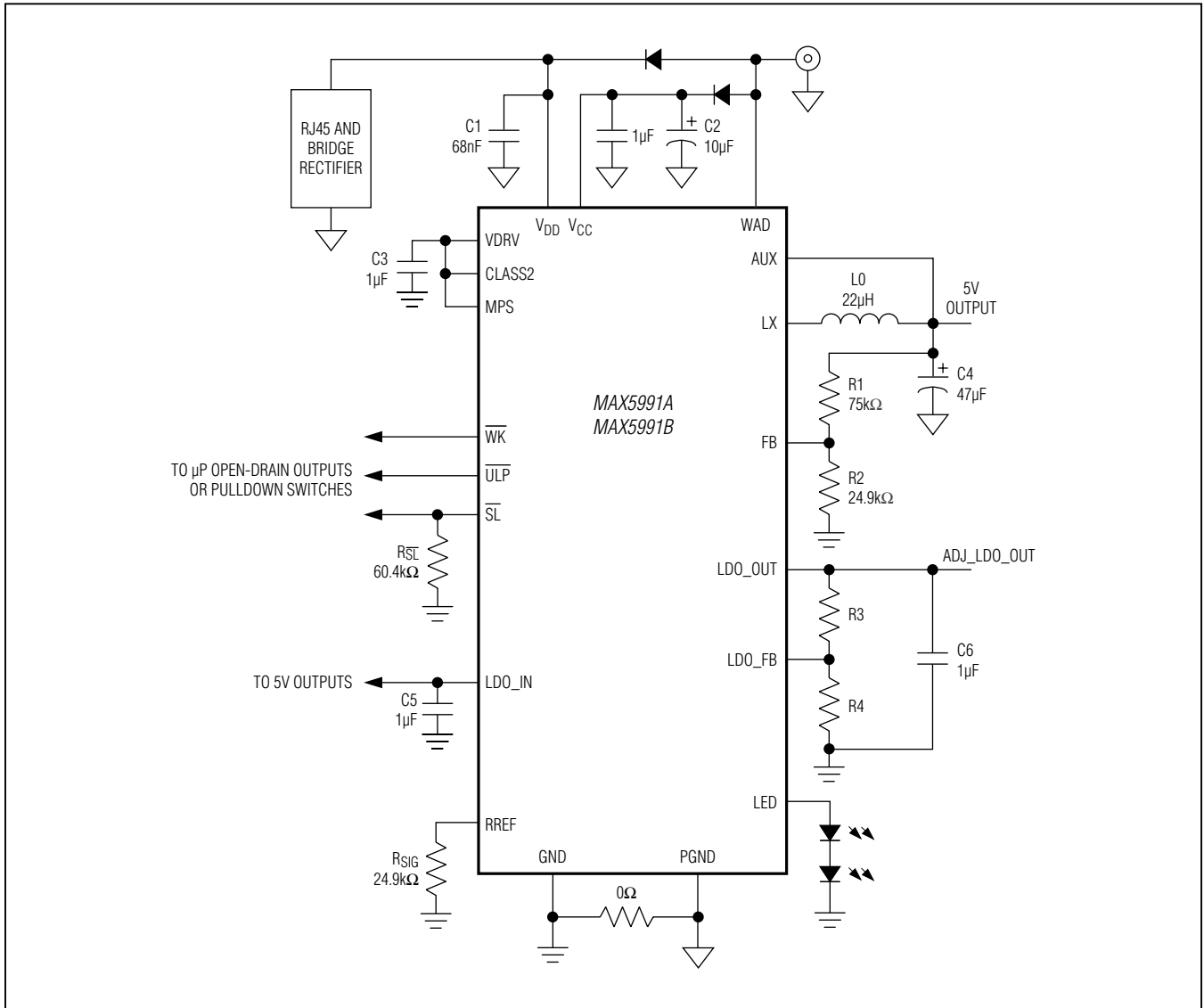
Figure 4. MAX5991A/MAX5991B 5V Buck Regulator and Adjustable LDO
