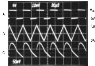
MEDIUM-LOAD SWITCHING WAVEFORMS ( V_{OUT} = 5\text{V} )
