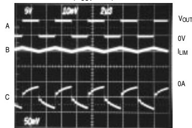
HEAVY-LOAD SWITCHING WAVEFORMS ( V_{OUT} = 5\text{V} )
