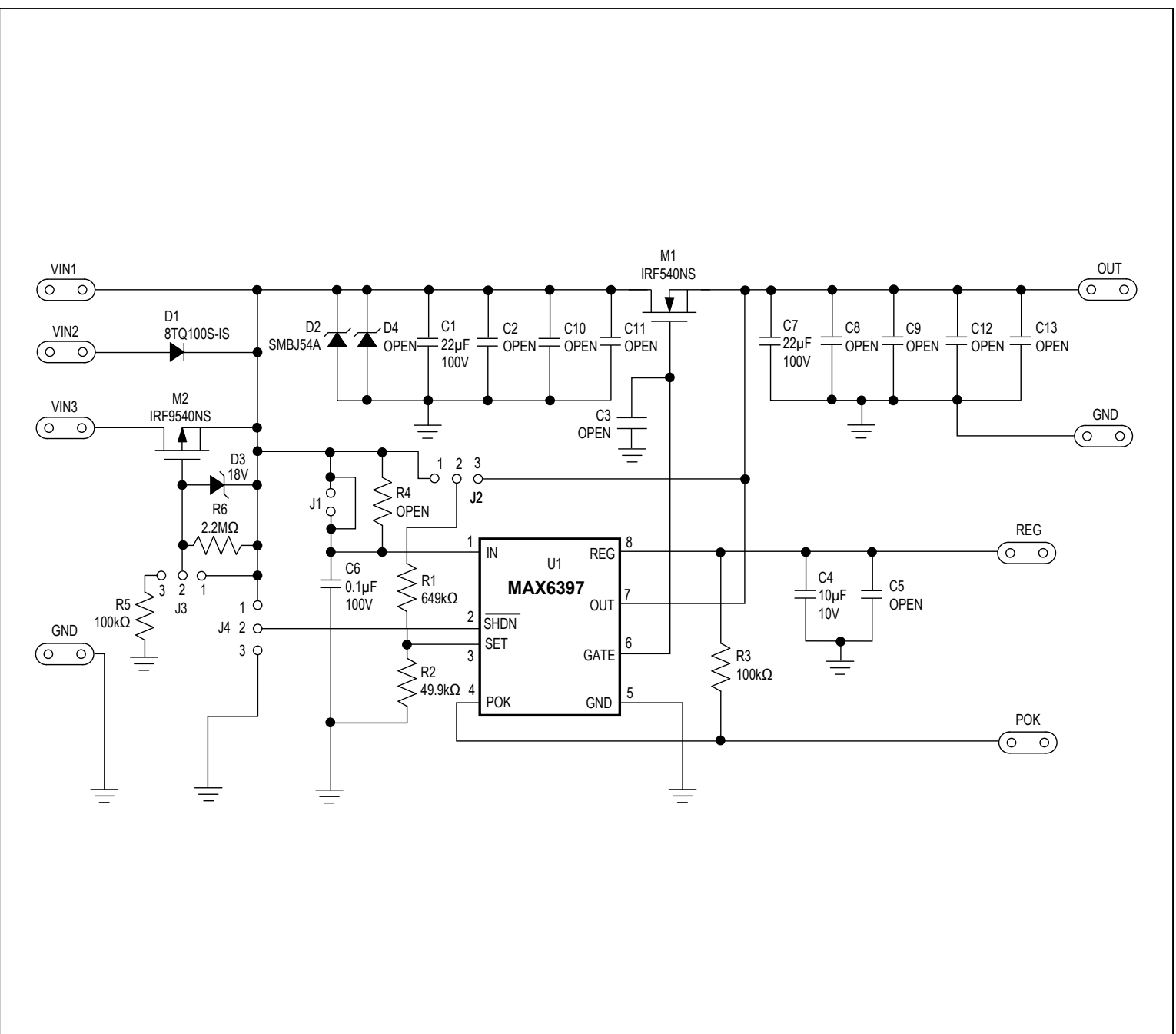
Figure 1. MAX6397 EV Kit Schematic
