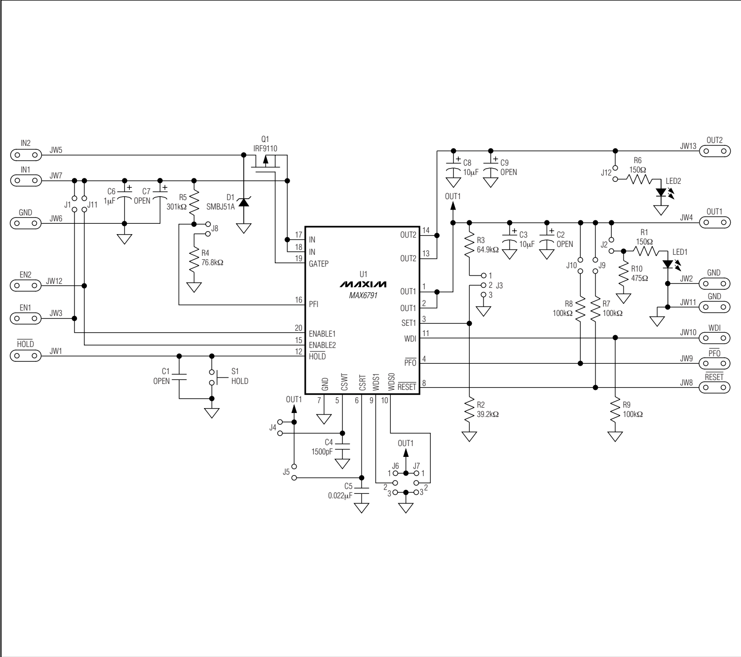
Figure 1. MAX6791 EV Kit Schematic
