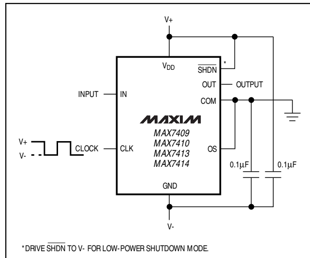
Figure 4. Dual-Supply Operation
