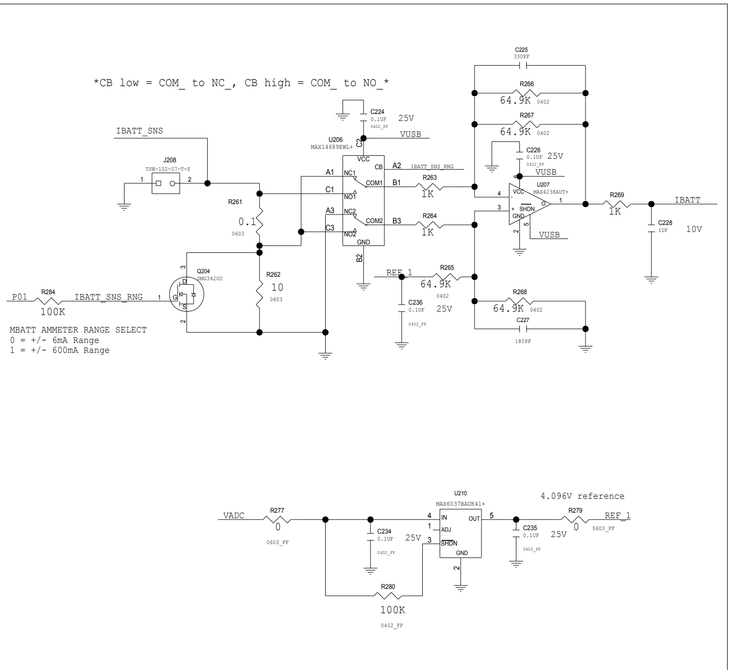
Figure 13. MAX77650/MAX77651 EV Kit Schematic (5 of 6)
