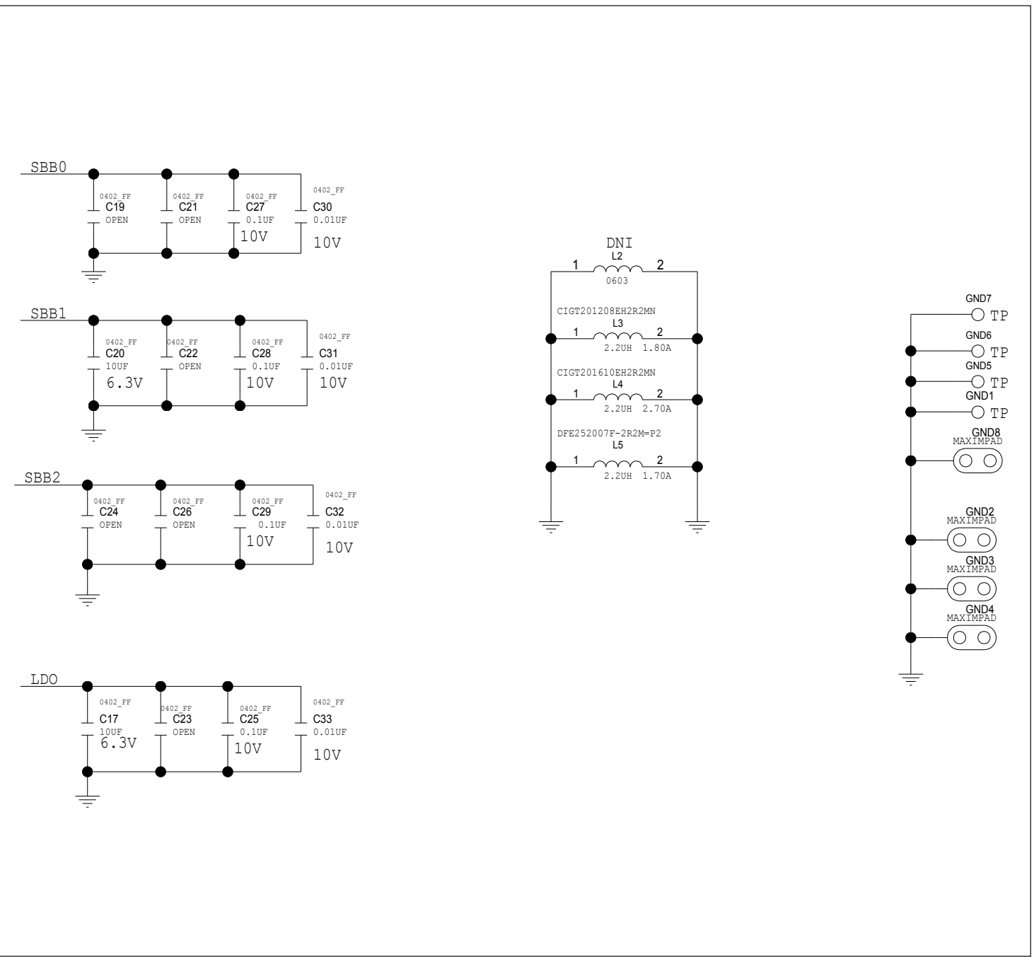
Figure 11. MAX77650/MAX77651 EV Kit Schematic (3 of 6)
