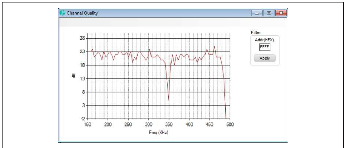
Figure 2. Channel Quality Analyzer Showing Strong 350kHz Interference
