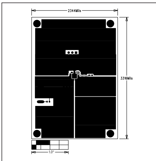
Figure 3. MAX8556 EV Kit PC Board Layout—Component Side
