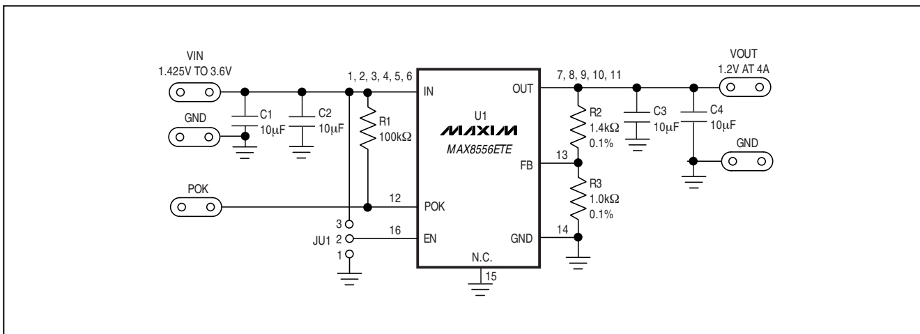
Figure 1. MAX8556 EV Kit Schematic
