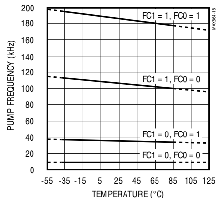
PUMP FREQUENCY vs. TEMPERATURE
