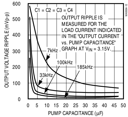
OUTPUT VOLTAGE RIPPLE vs. PUMP CAPACITANCE ( V_{IN} = 3.15V , V_+ + |V_-| = 10V )
