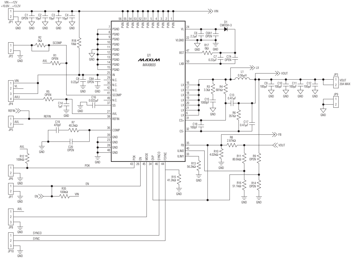
Figure 1a. MAX8655 EV Kit Schematic (Sheet 1 of 2)
