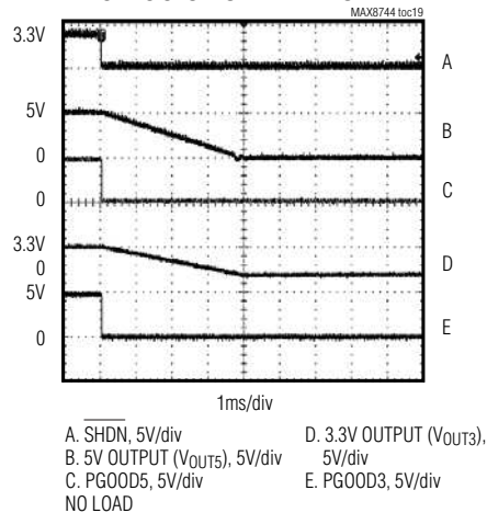
SMPS SHUTDOWN WAVEFORM
