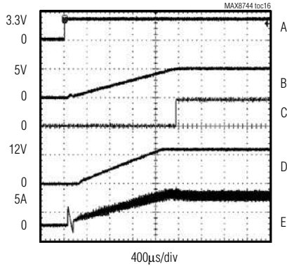
SOFT-START WAVEFORM
