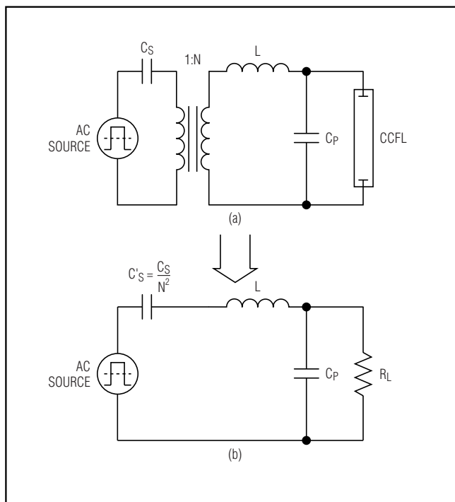
Figure 5. Equivalent Resonant Tank Circuit
