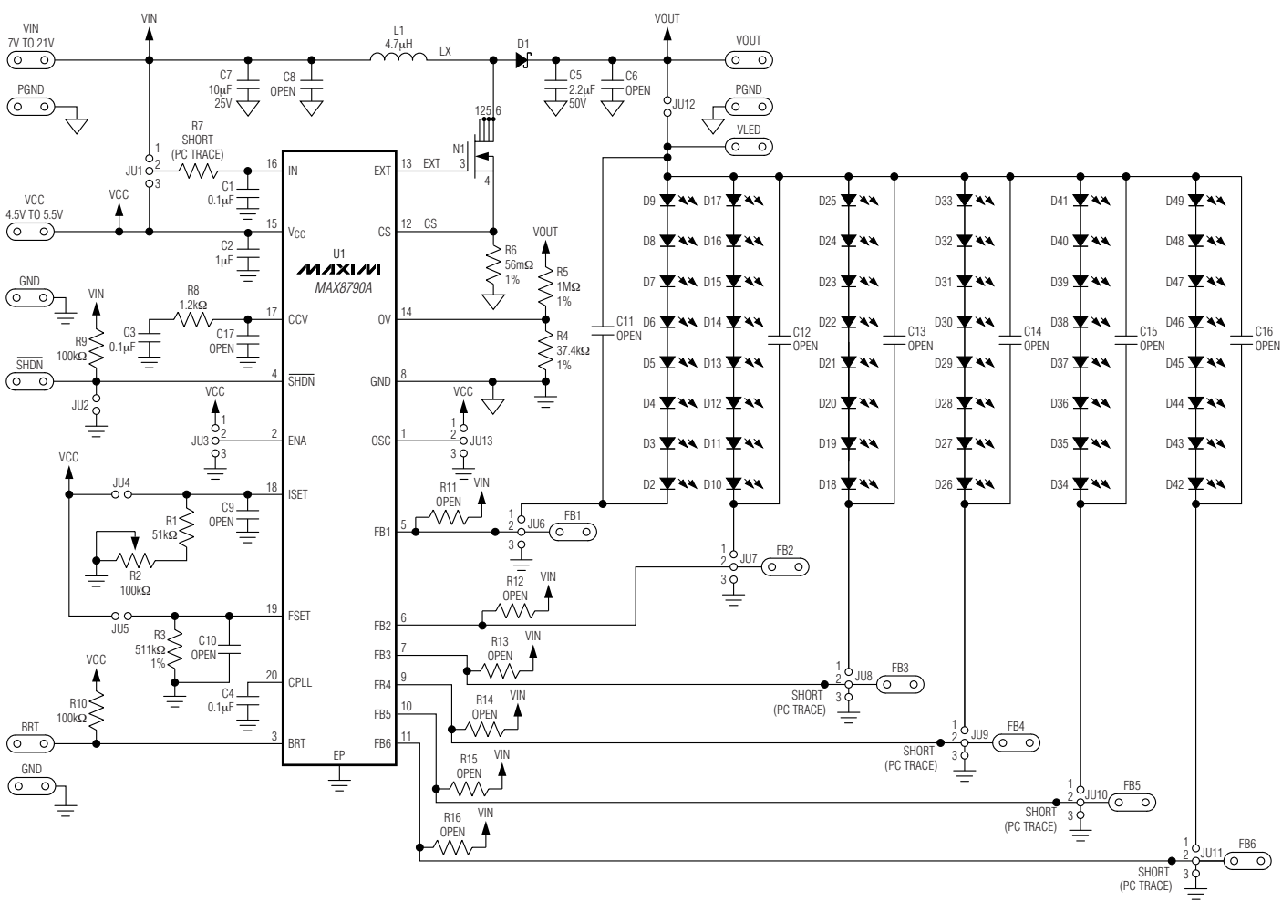
Figure 1. MAX8790A EV Kit Schematic
