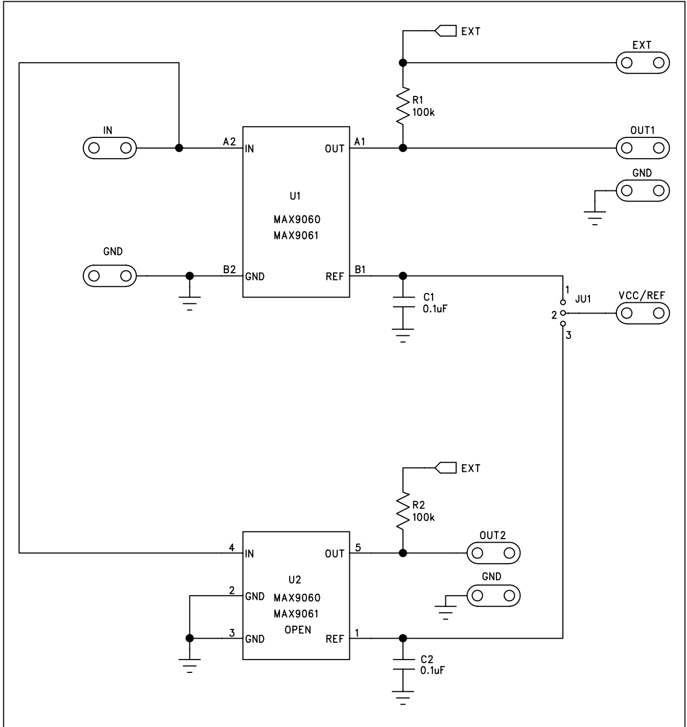
Figure 1. MAX9060/MAX9061 EV Kits Schematic
