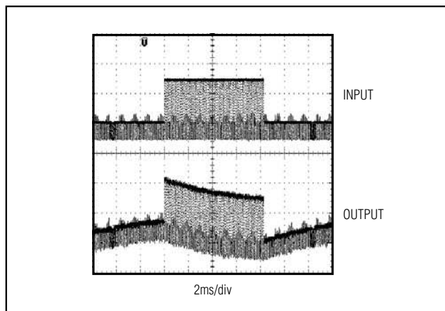
Figure 1. AC-Coupled Output
