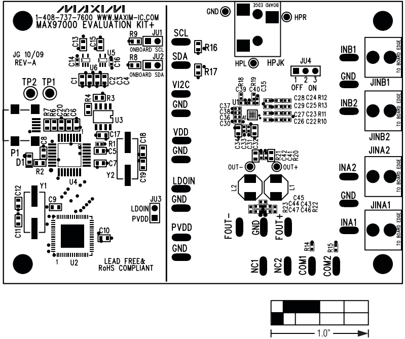
Figure 5. MAX97000 EV Kit Component Placement Guide—Component Side
