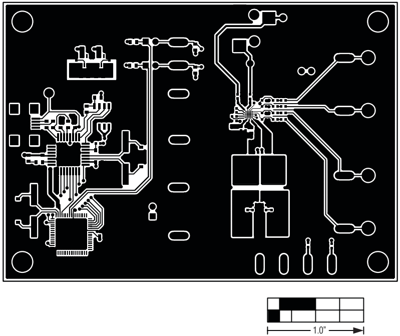
Figure 6. MAX97000 EV Kit PCB Layout—Component Side
