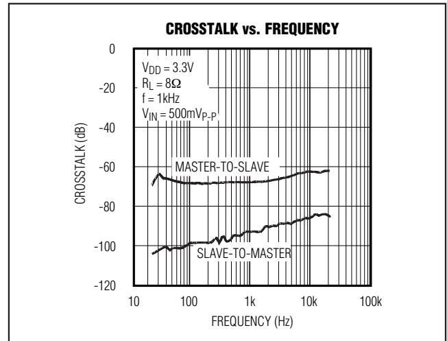
Figure 9. Master-Slave Crosstalk
