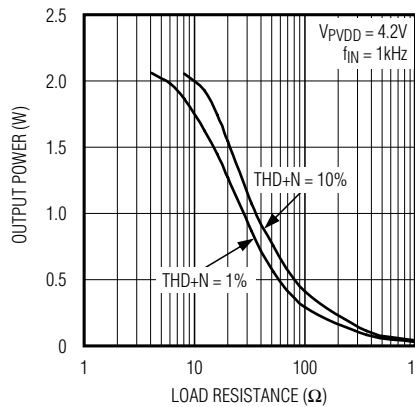
OUTPUT POWER vs. LOAD RESISTANCE (MAX98308)
