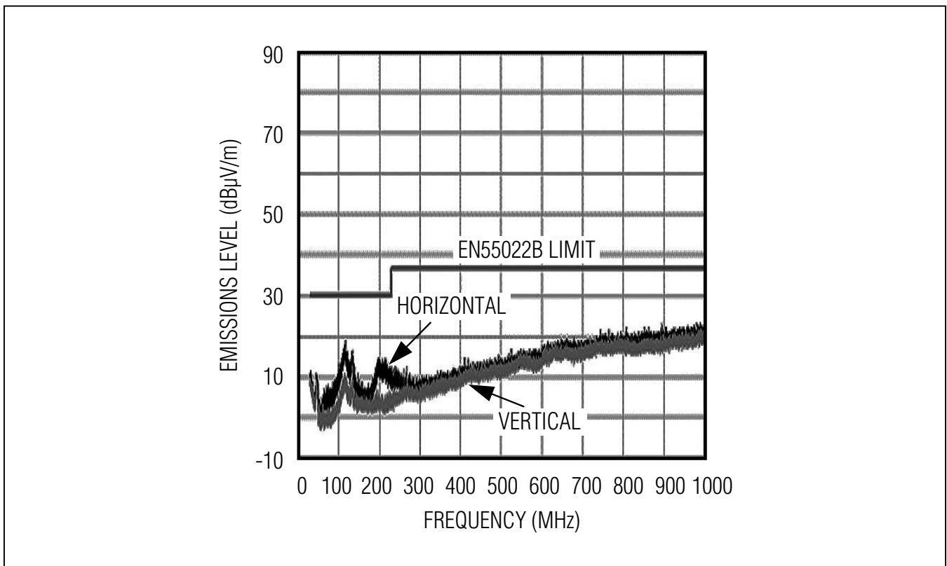
Figure 3. EMI Performance with V_{PDD} = 5V , 12in of Speaker Cable, No Output Filter
