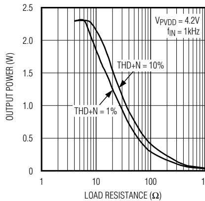
OUTPUT POWER vs. LOAD RESISTANCE (MAX98307)
