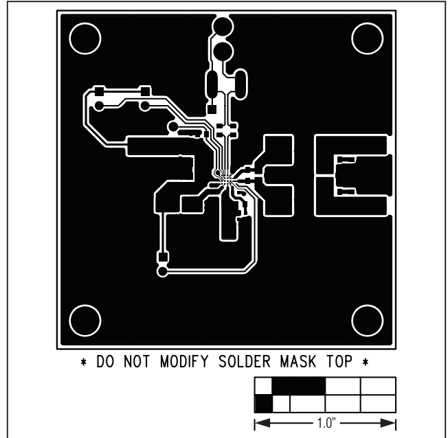
Figure 3. MAX98500 EV Kit PCB Layout—Component Side
