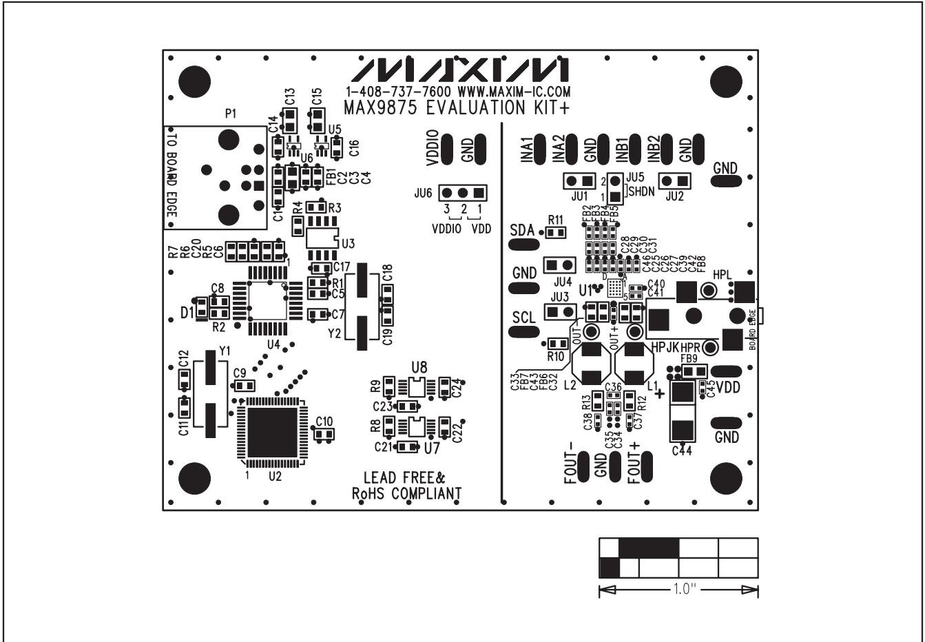
Figure 5. MAX9875 EV Kit Component Placement Guide—Component Side
