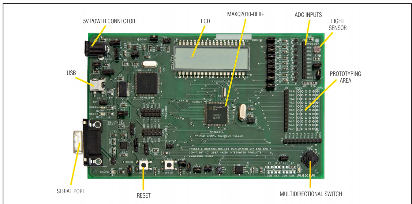
Figure 1. MAXQ2010 EV Kit Board
