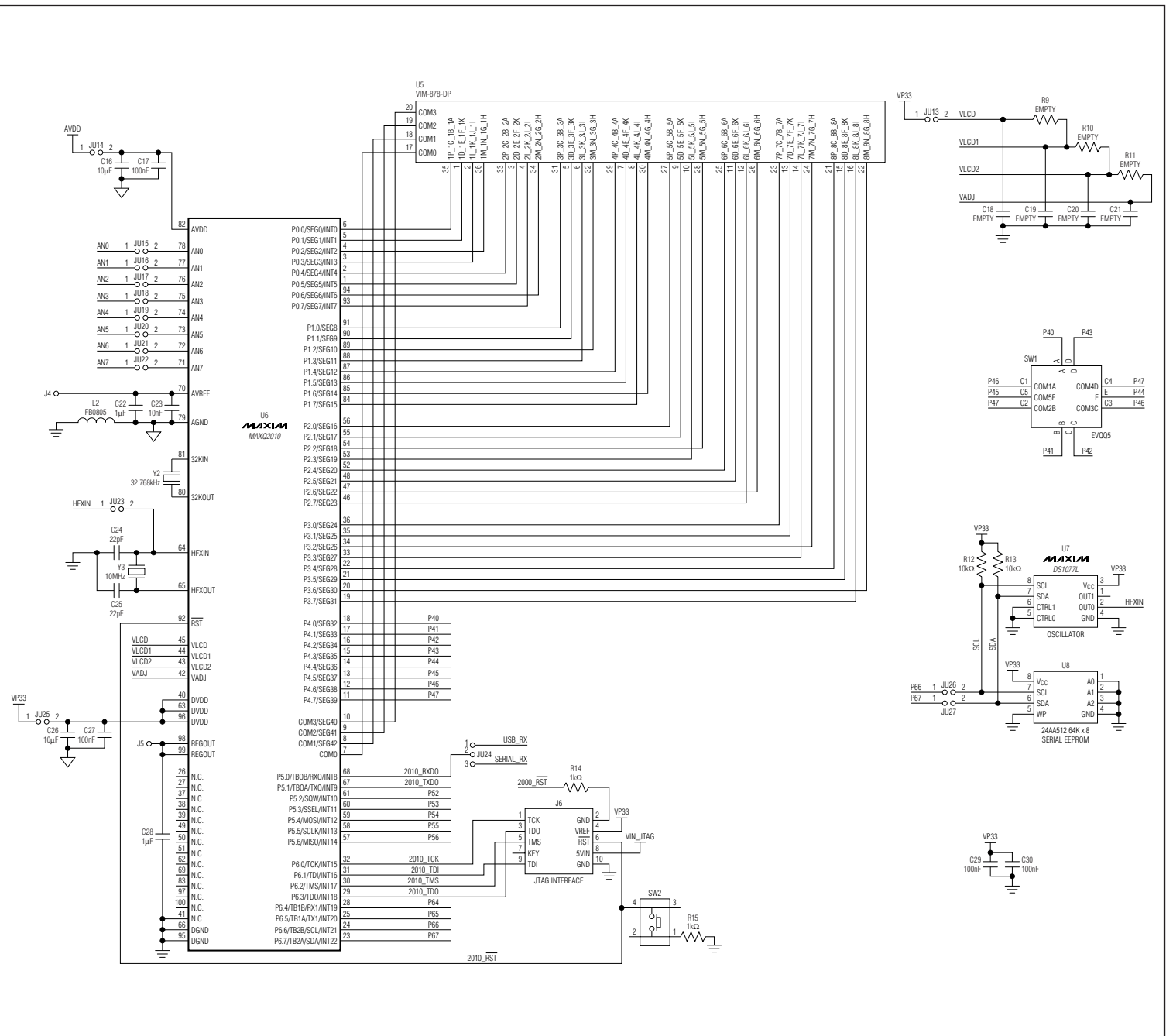
Figure 6. MAXQ2010 EV Kit Schematic—Microcontroller/LCD (2 of 3)
