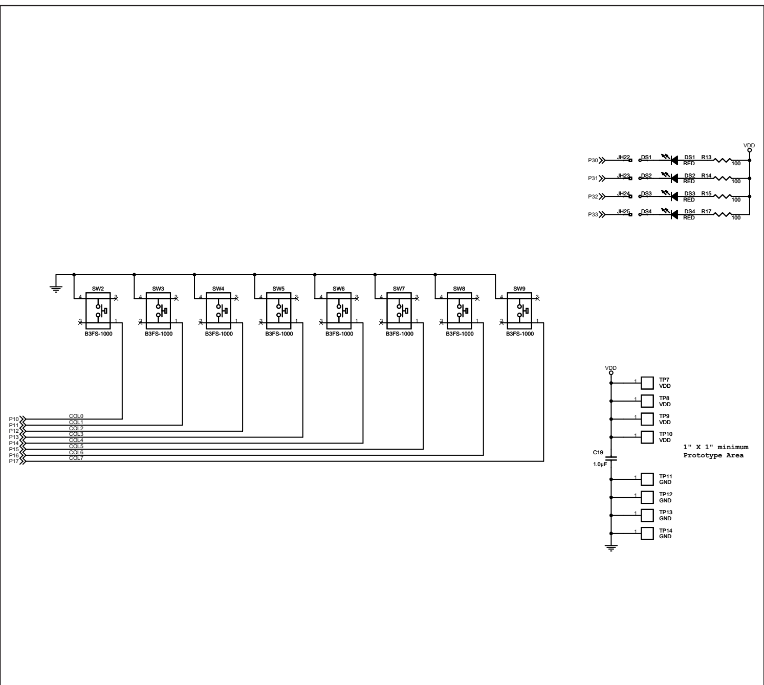
Figure 3b. MAXQ610 EV Kit Board Schematic—Pushbuttons (Sheet 2 of 2)
