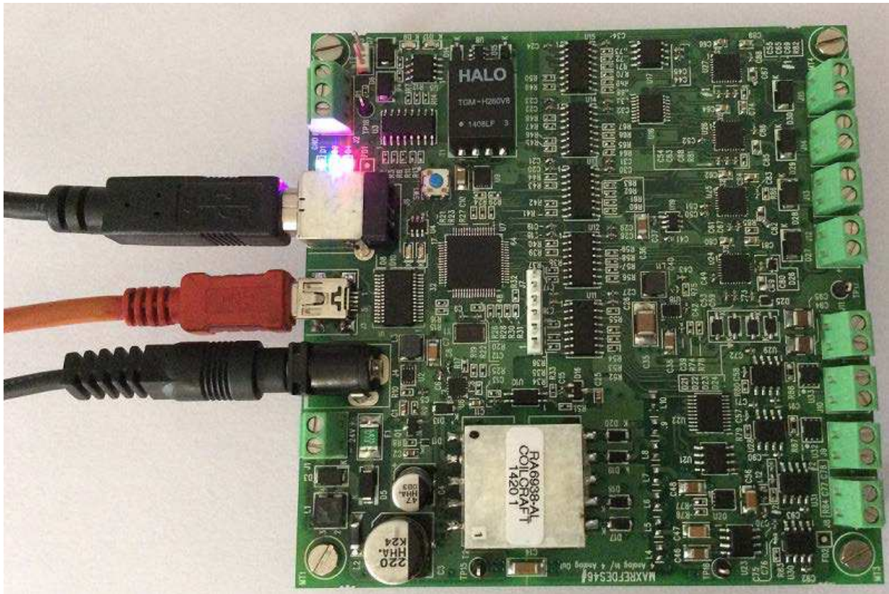
Figure 1. MAXREFDES46# board.
