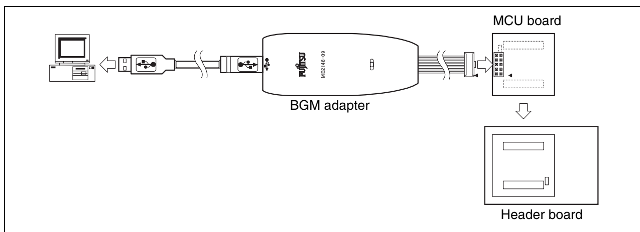
Figure 1 System Configuration
