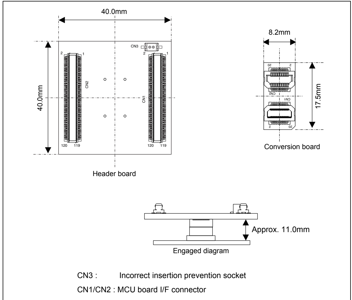
Figure 4-1. Header board and conversion board dimensions
