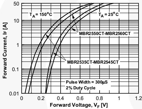
Figure 3. Forward Voltage Characteristics, per Leg
