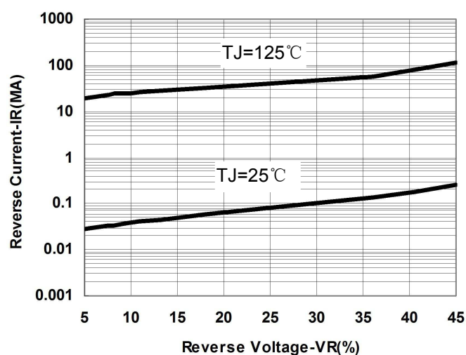
Fig.2-Typical Reverse Characteristics
