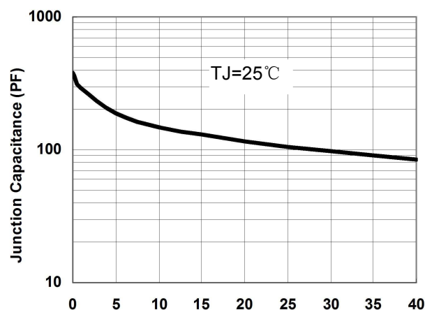
Fig.1-Typical Junction Capacitance
