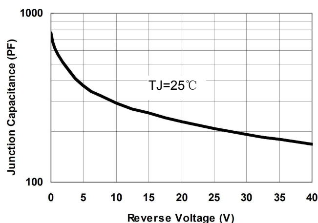
Fig.1-Typical Junction Capacitance
