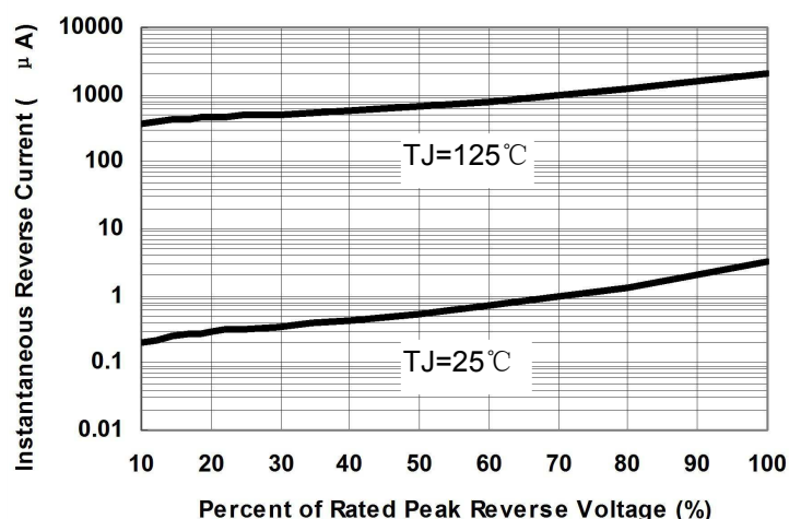
Fig.2-Typical Reverse Characteristics
