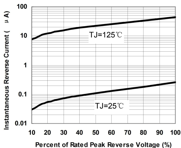
Fig.2-Typical Reverse Characteristics
