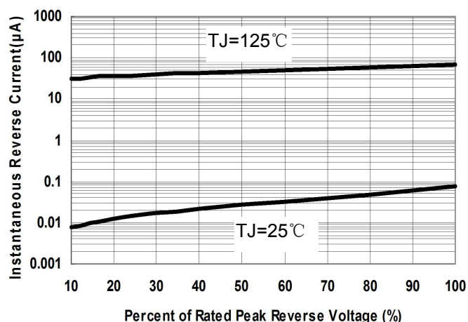
Fig.2-Typical Reverse Characteristics
