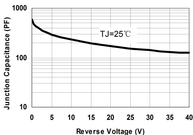
Fig.1-Typical Junction Capacitance
