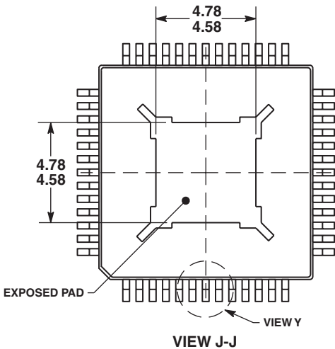
VIEW J-J
