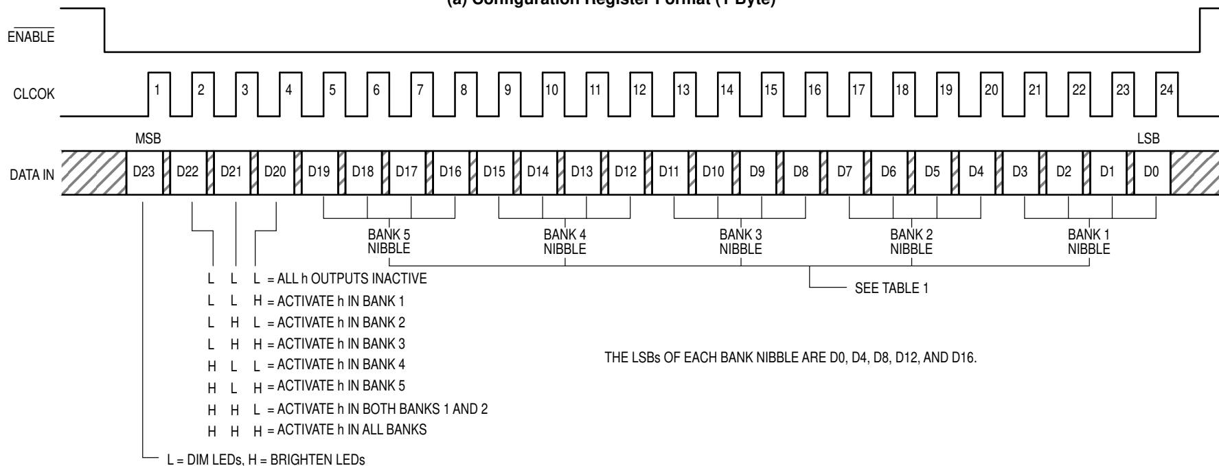
Figure 8. Timing Diagrams for Non-Cascaded Devices
