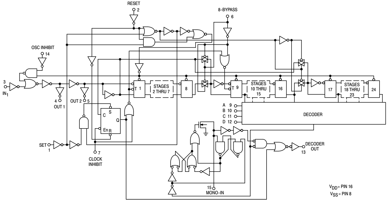
LOGIC DIAGRAM
