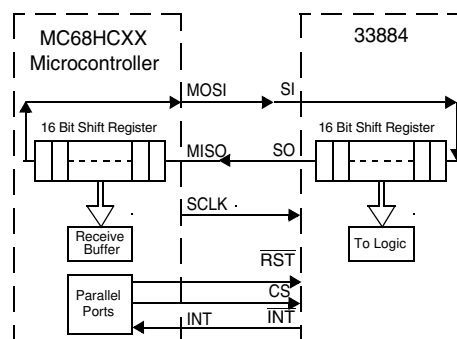
Figure 4. SPI Interface with Microprocessor
