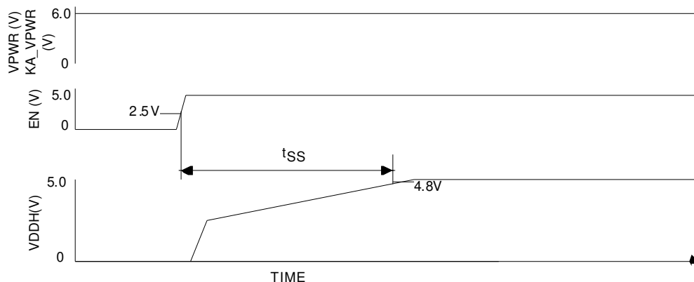
Figure 4. Soft-Start Time
