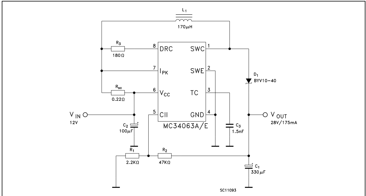
Figure 13. Step-up converter
