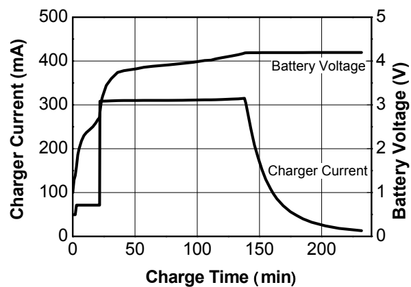
Figure 17. USB Charger Complete Charge Cycle V_{USB}=5.0 V, R_{IUSB}=6.52 k \Omega , 740 mA Battery, T_A=25^\circ C
