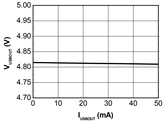
Figure 24. V_{USBOUT} vs I_{USBOUT} V_{USB}=5.0 V, T_A=25^\circ\text{C}
