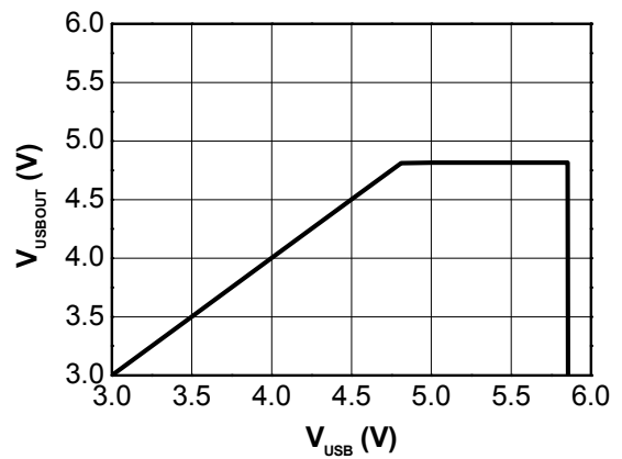
Figure 25. V_{USBOUT} vs V_{USB} I_{USBOUT}=0 mA, T_A=25^\circ\text{C}
