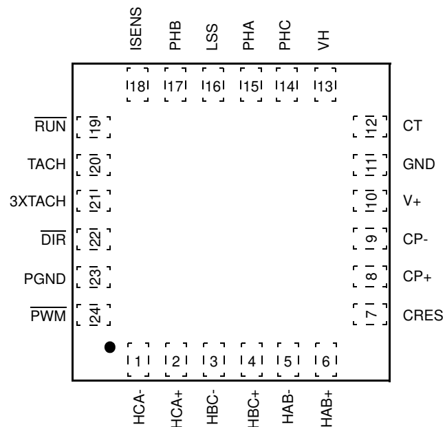
Figure 3. 34929 Pin Connections
