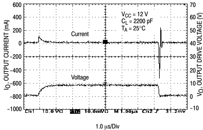
Figure 6. Output Waveform
