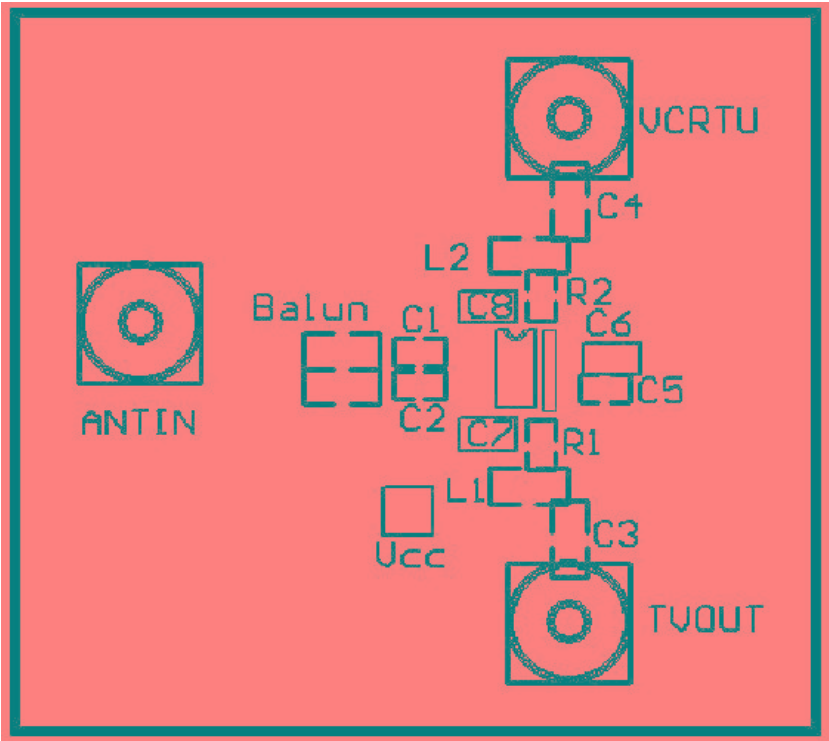
Figure 4. Proposed Single-Sided PCB Layout
