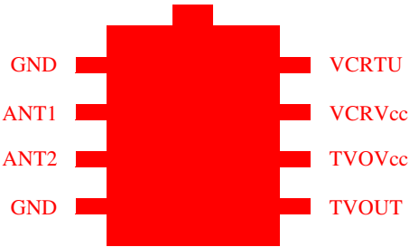
Figure 1. Pin Connections
