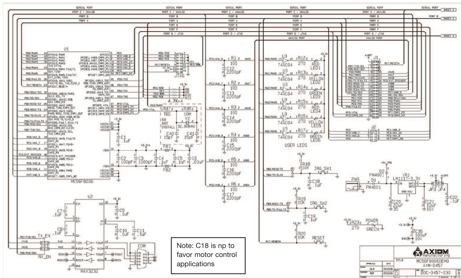
Figure A-1. MC56F8006DEMO Schematic: Part 1
