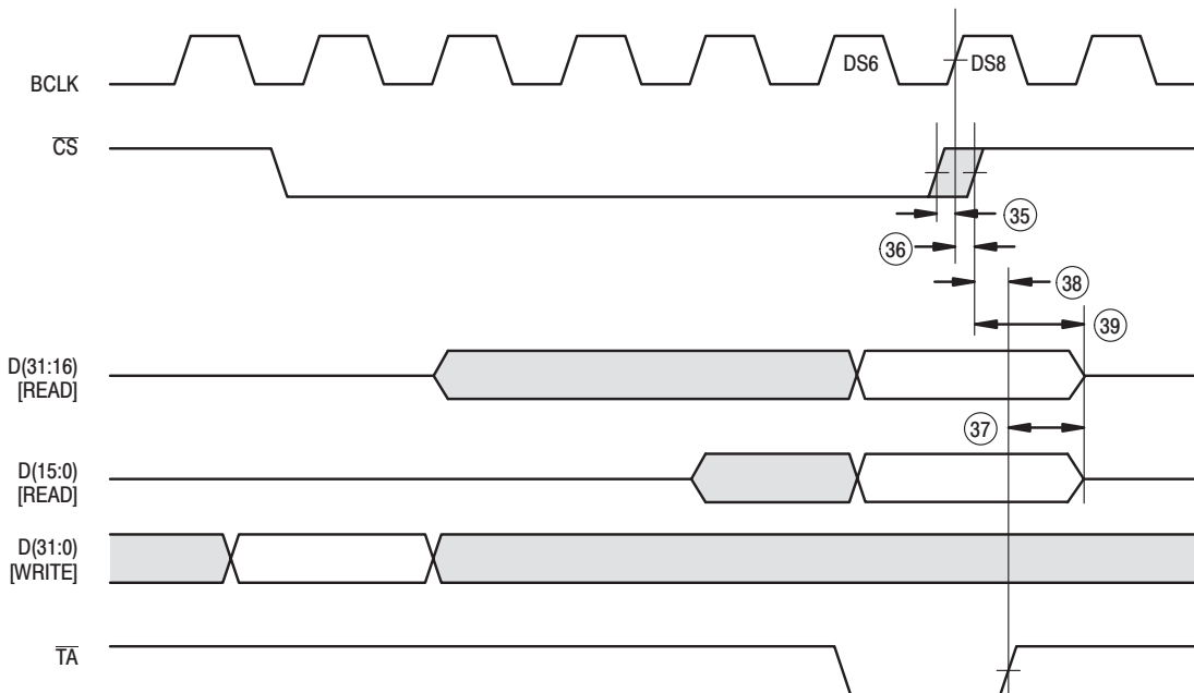
Figure 8. MC68150 READ/WRITE Timing Asynchronous Termination
