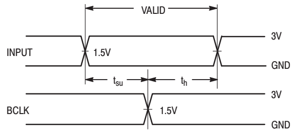
Figure 11. Setup/Hold Times
